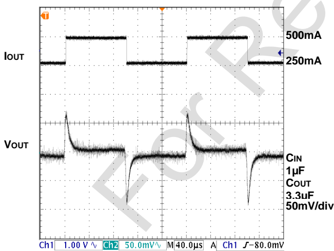
LOAD TRANSIENT
