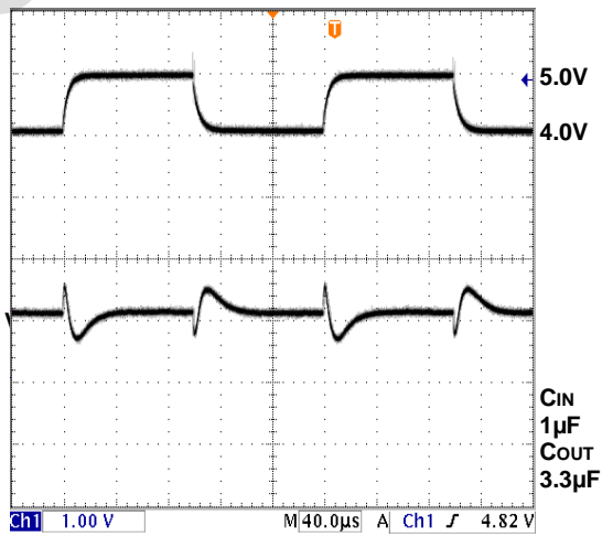
LINE TRANSIENT (I OUT =10mA)
